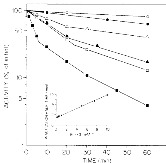
FIGURE 1: Inactivation of isocitrate dehydrogenase by 1.0 mM (■) and 0.1 (□) bromoketoglutarate (Br-kG) in the absence of other ligands and by 0.1 mM bromoketoglutarate in the presence of 1 mM \alpha -ketoglutarate (▲), 0.3 mM \text{MnCl}_2 (△), 1 mM DL-isocitrate (●), or 0.1 mM NADP (○). Dependency of inactivation rate of isocitrate dehydrogenase on the reciprocal of bromoketoglutarate (Br-kG) concentration is shown in the inset. For details, see Experimental Procedures.
